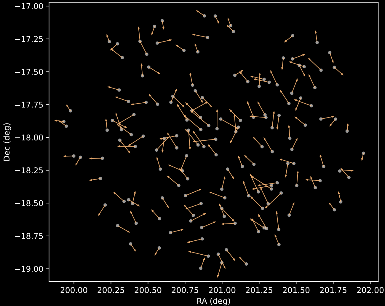
GALAH DR4 Cluster 3 Proper Motion Vectors (n=154)
