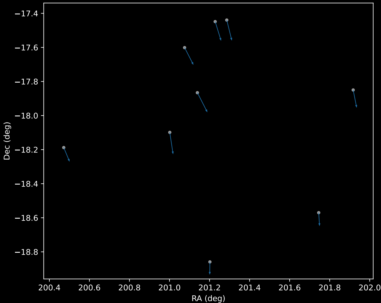
GALAH DR4 Cluster 0 Proper Motion Vectors (n=9)
