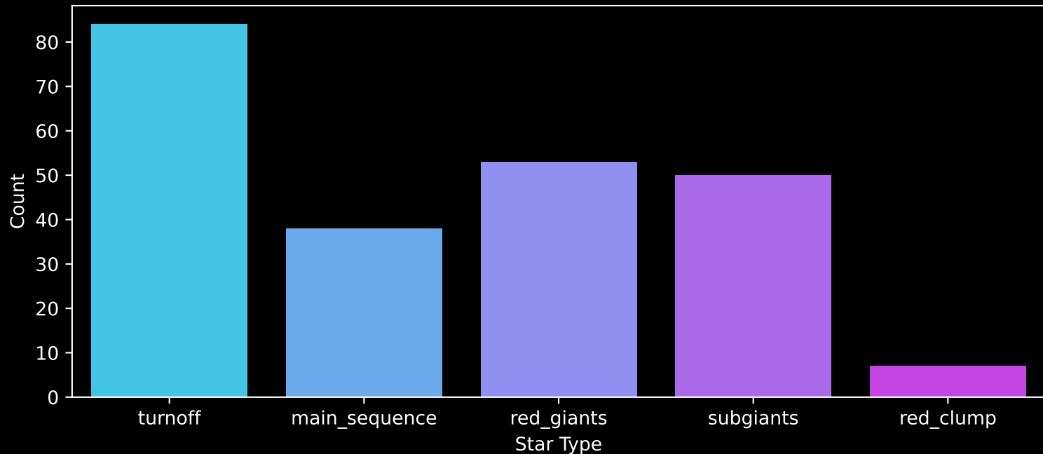
GALAH DR4 Field: [8613] Count plot of Star Type
