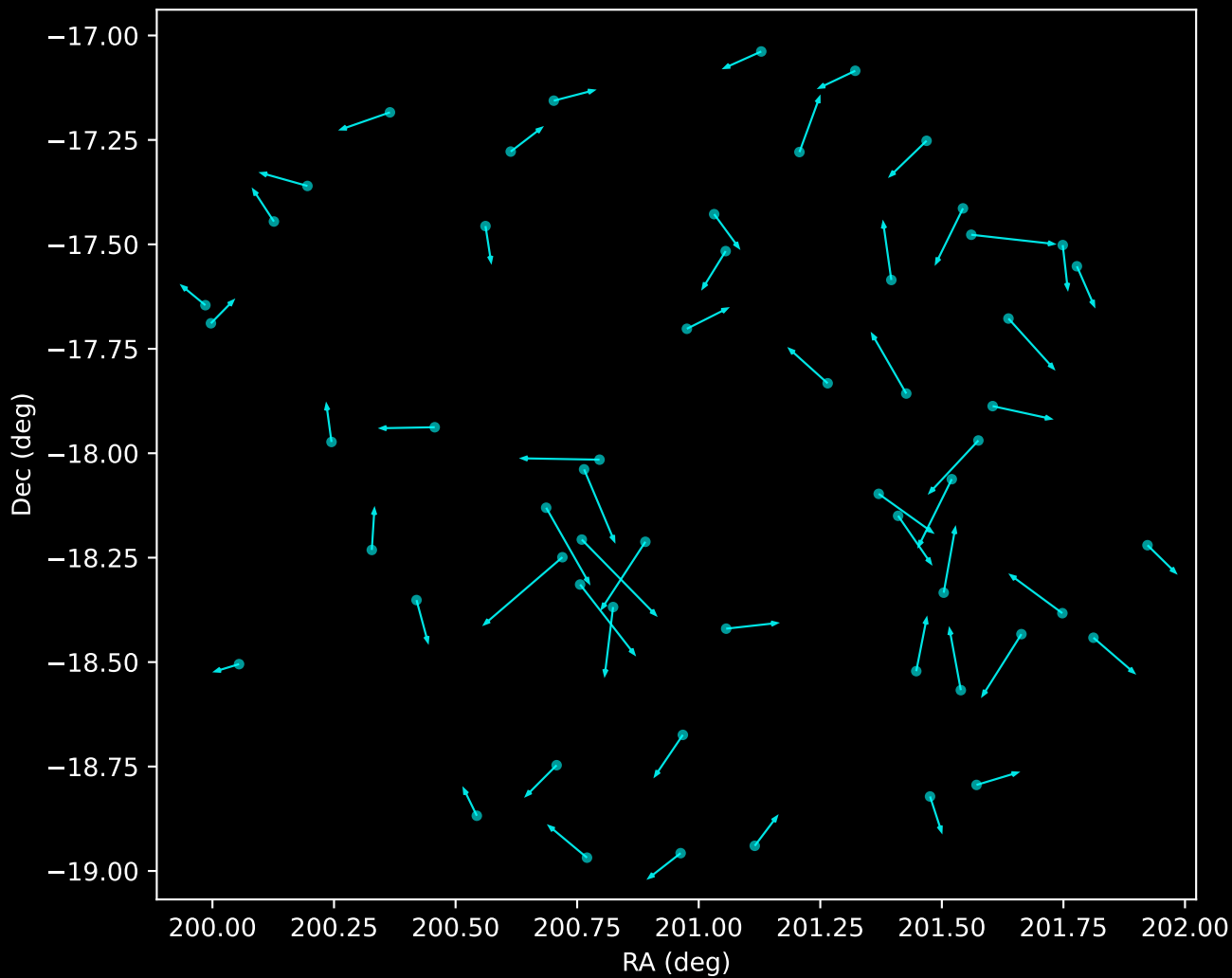
GALAH DR4 Noise Stream Proper Motion Vectors (n=57)
