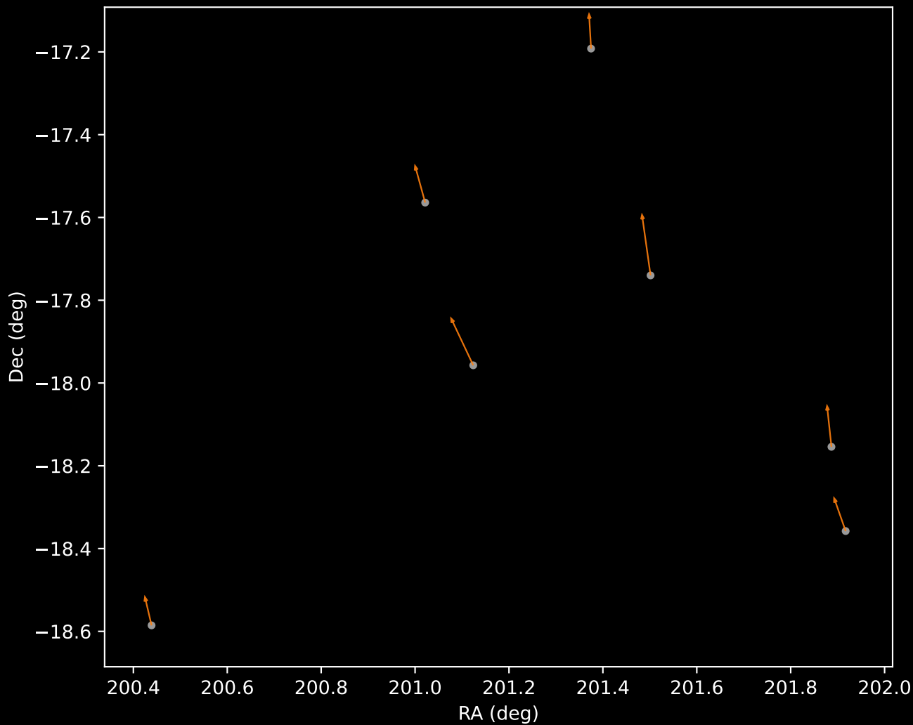
GALAH DR4 Cluster 2 Proper Motion Vectors (n=7)
