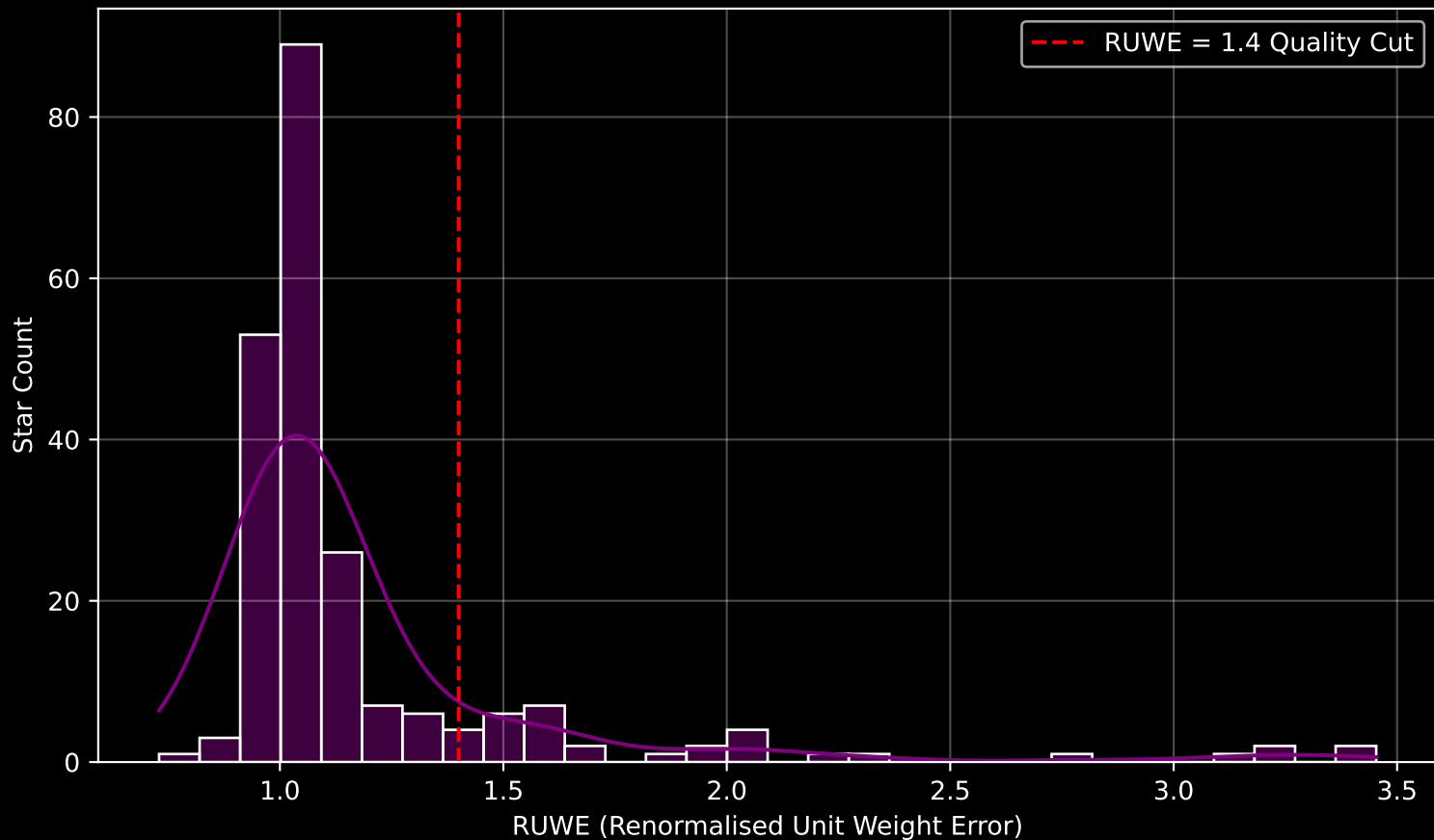
GALAH DR4 Field [8613] RUWE Distribution (n= 219)
